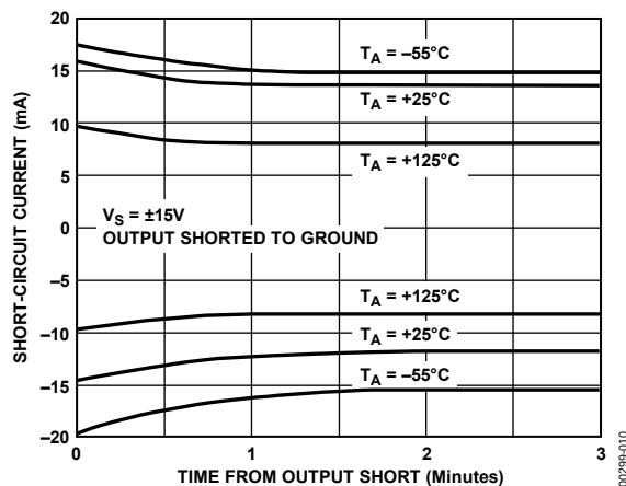
Figure 10. Short-Circuit Current vs. Time, Temperature
