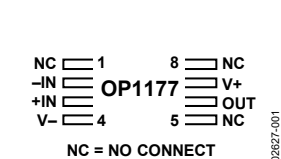
Figure 1. 8-Lead MSOP (RM Suffix)
