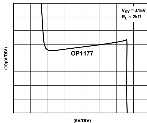
Figure 51. Gain Linearity
