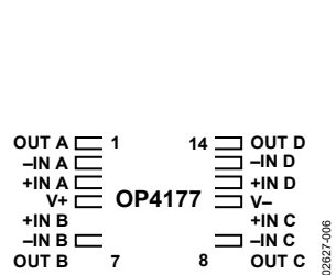
Figure 6. 14-Lead TSSOP (RU Suffix)
