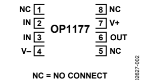
Figure 2. 8-Lead SOIC_N (R Suffix)
