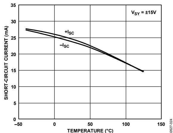
Figure 24. Short-Circuit Current vs. Temperature
