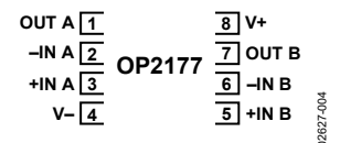
Figure 4. 8-Lead SOIC_N (R Suffix)
