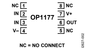
Figure 2. 8-Lead SOIC_N (R Suffix)
