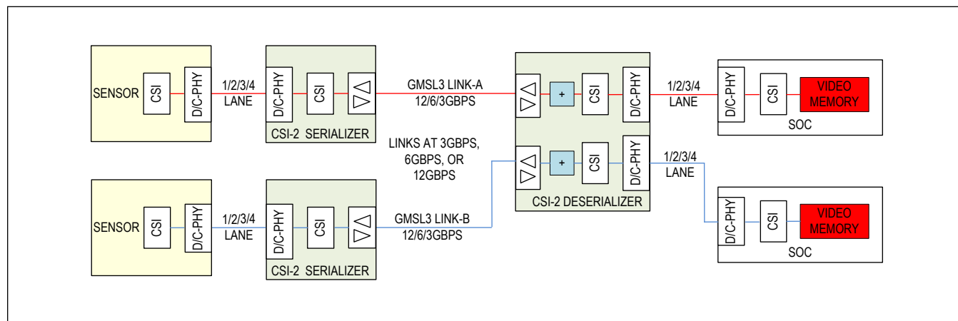
Figure 21. Dual Link, Separate Data
