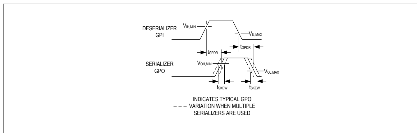
Figure 10. GPI-to-GPO Delay and Skew
