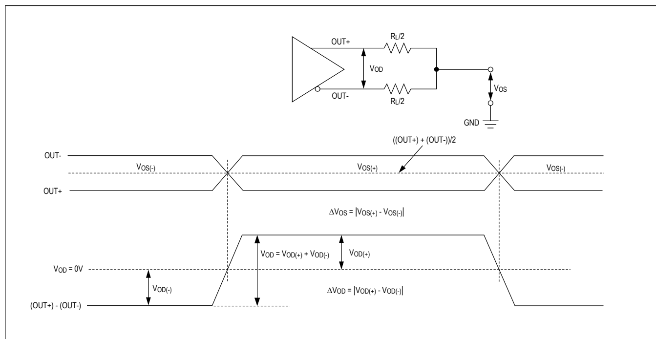
Figure 2. GMSL3 Reverse-Channel Serial Outputs
