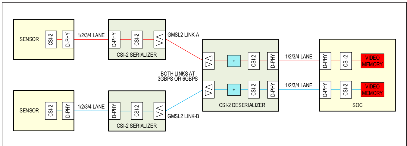
Figure 20. Independent GMSL2 Links with Dedicated Outputs
