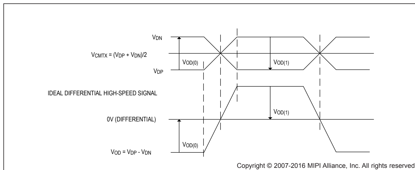
Figure 3. Ideal Single-ended and Resulting Differential HS Signals
