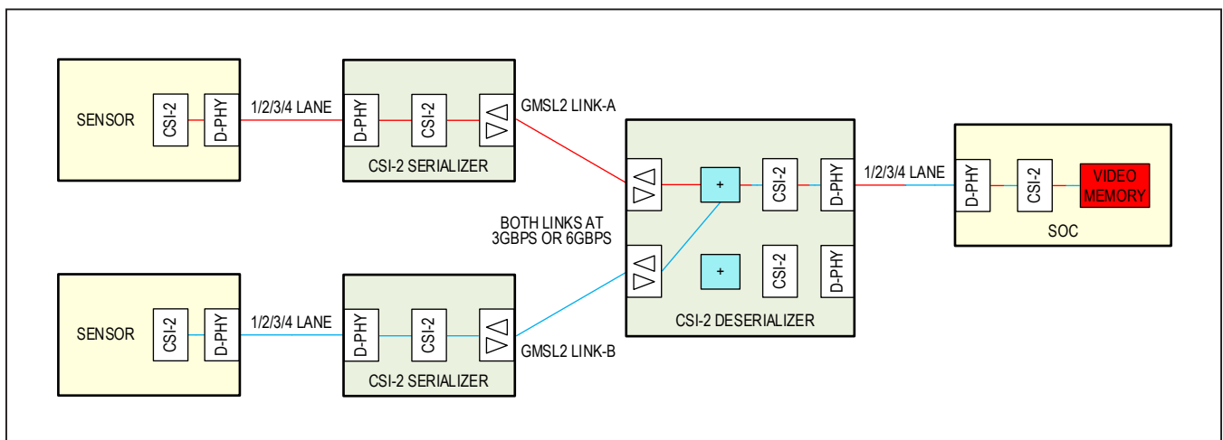
Figure 21. Independent GMSL2 Links with Aggregated Output
