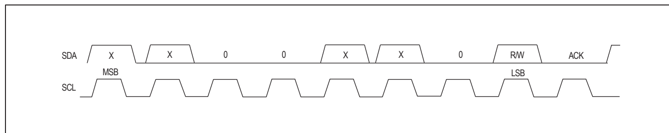
Figure 30. Subordinate Address
