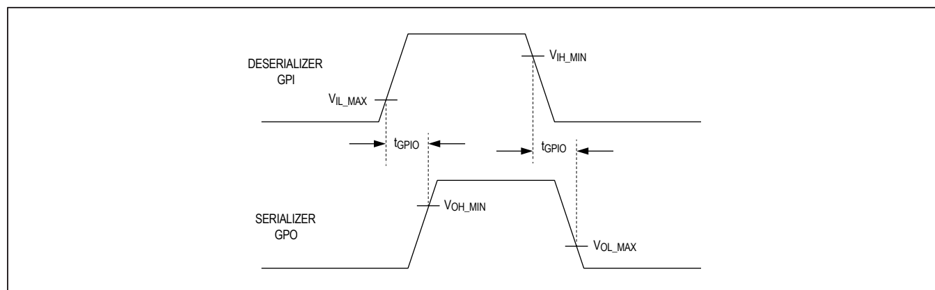
Figure 9. GPI-to-GPO Delay
