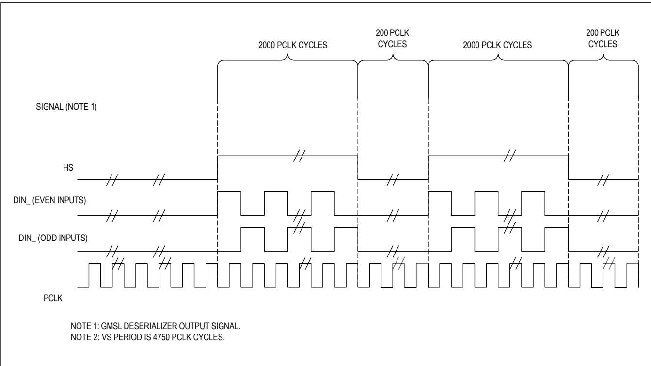
Figure 5. Worst-Case Pattern Input
