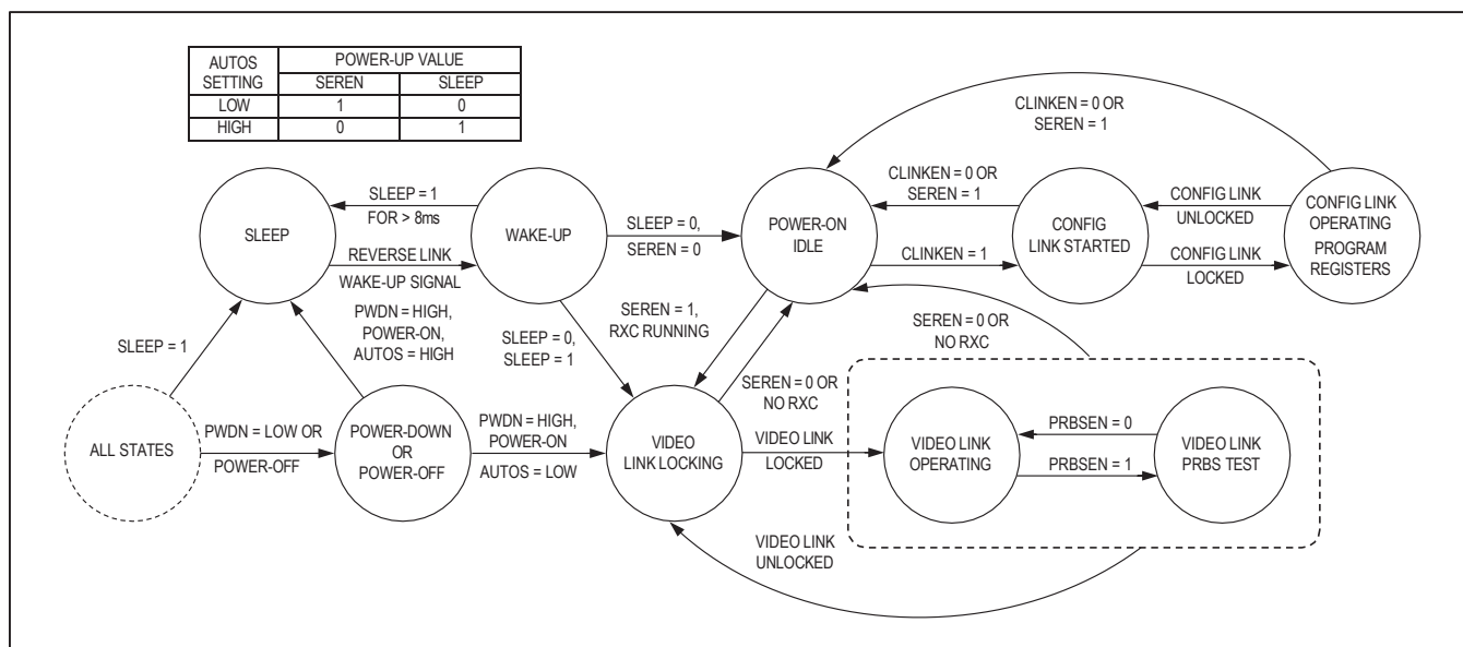
Figure 37. State Diagram, CDS = High (Image Sensing)
