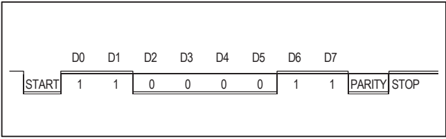
Figure 24. ACK Byte (0xC3)
