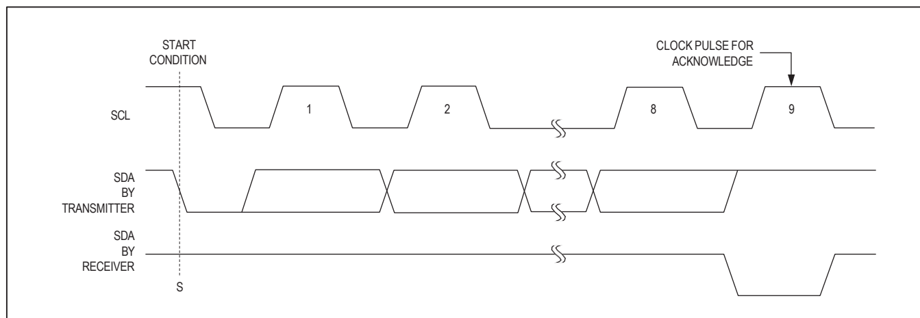
Figure 29. Acknowledge
