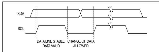
Figure 3. Bit Transfer
