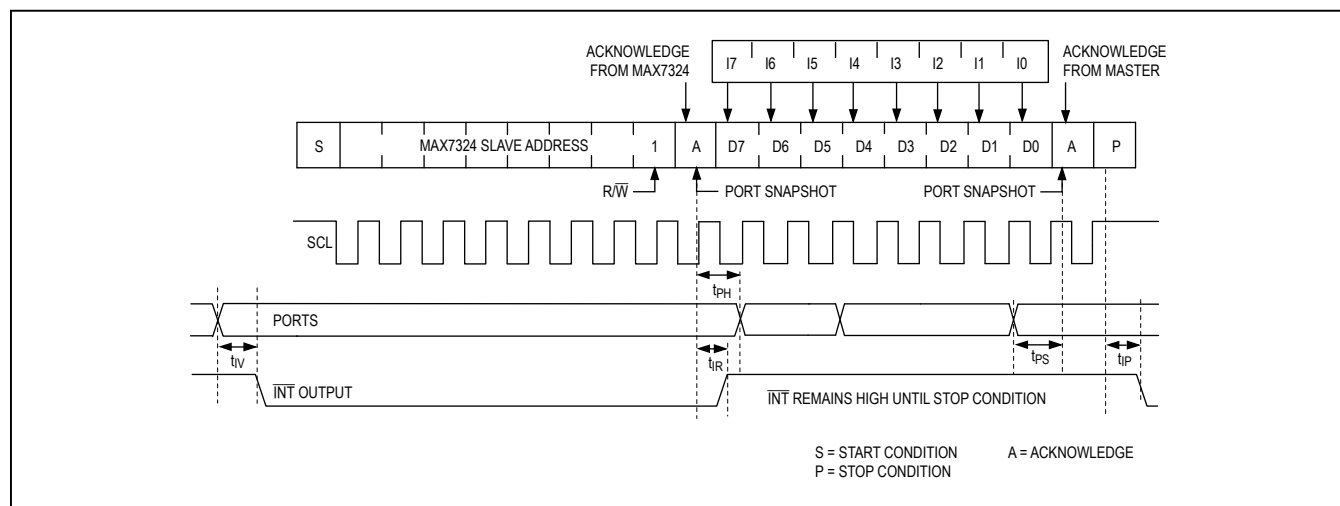
Figure 6. Reading Input Ports of the MAX7324 (1 Data Byte)
