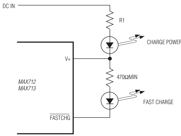
Figure 18. LED Connection for Status Outputs
