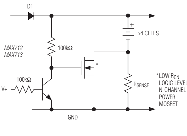
Figure 16. Shunting R_{SENSE} for Efficiency Improvement
