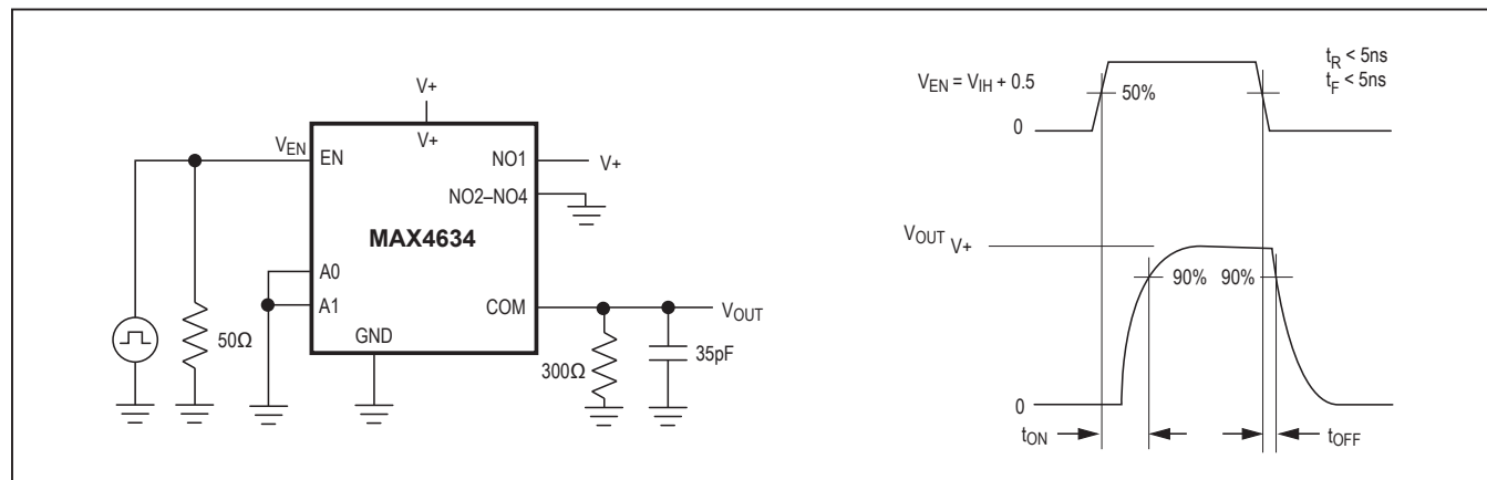
Figure 2. Switching Time
