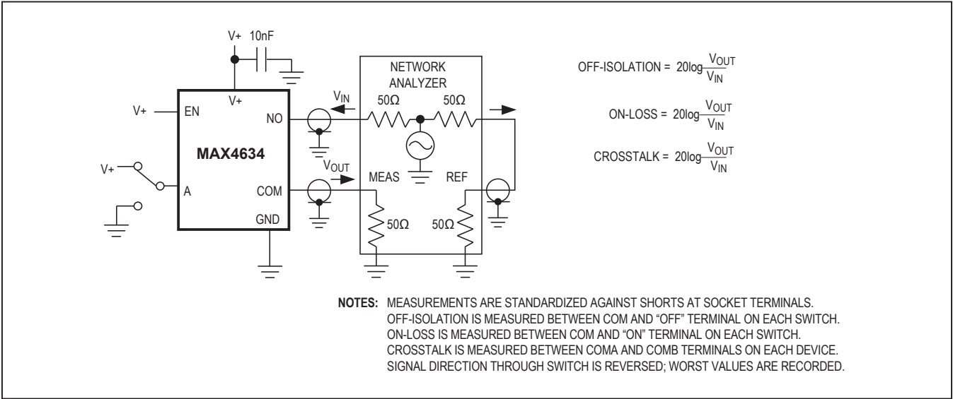
Figure 5. Off-Isolation/On-Channel Bandwidth
