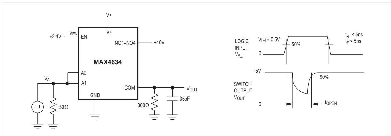
Figure 3. Break-Before-Make Interval
