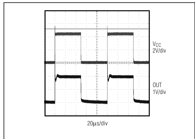
Figure 6. Power-Up/Power-Down Waveform
