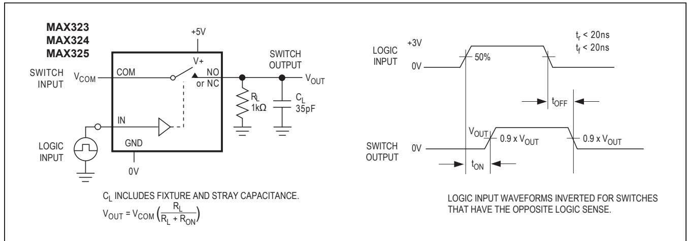
Figure 2. Switching Time
