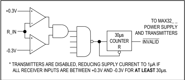
Figure 3a. MAX32__ Entering 1μA Supply Mode Through AutoShutdown
