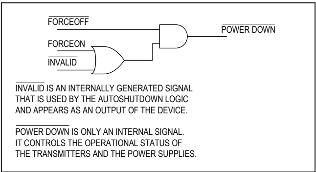
Figure 3c. AutoShutdown Logic
