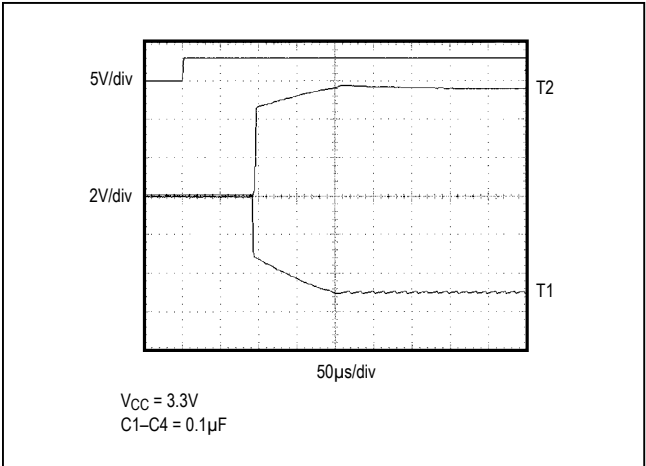
Figure 3. Transmitter Outputs when Exiting Shutdown or Powering Up
