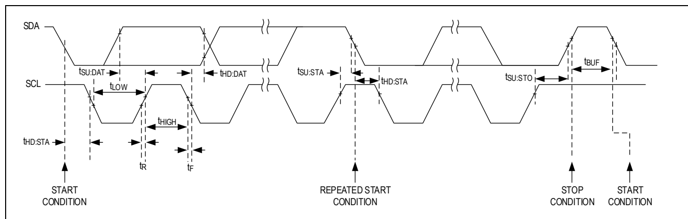
Figure 1. I^2\text{C}/\text{SMBus} Timing Diagram
