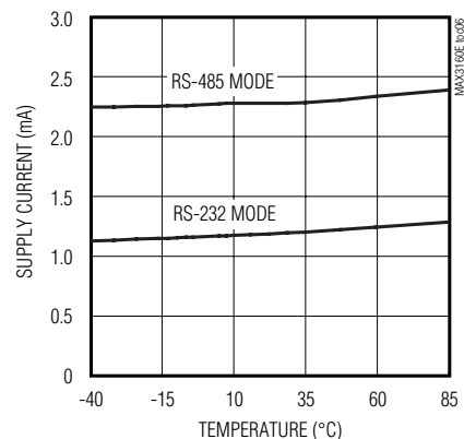
MAX3160E/MAX3161E NO-LOAD SUPPLY CURRENT vs. TEMPERATURE
