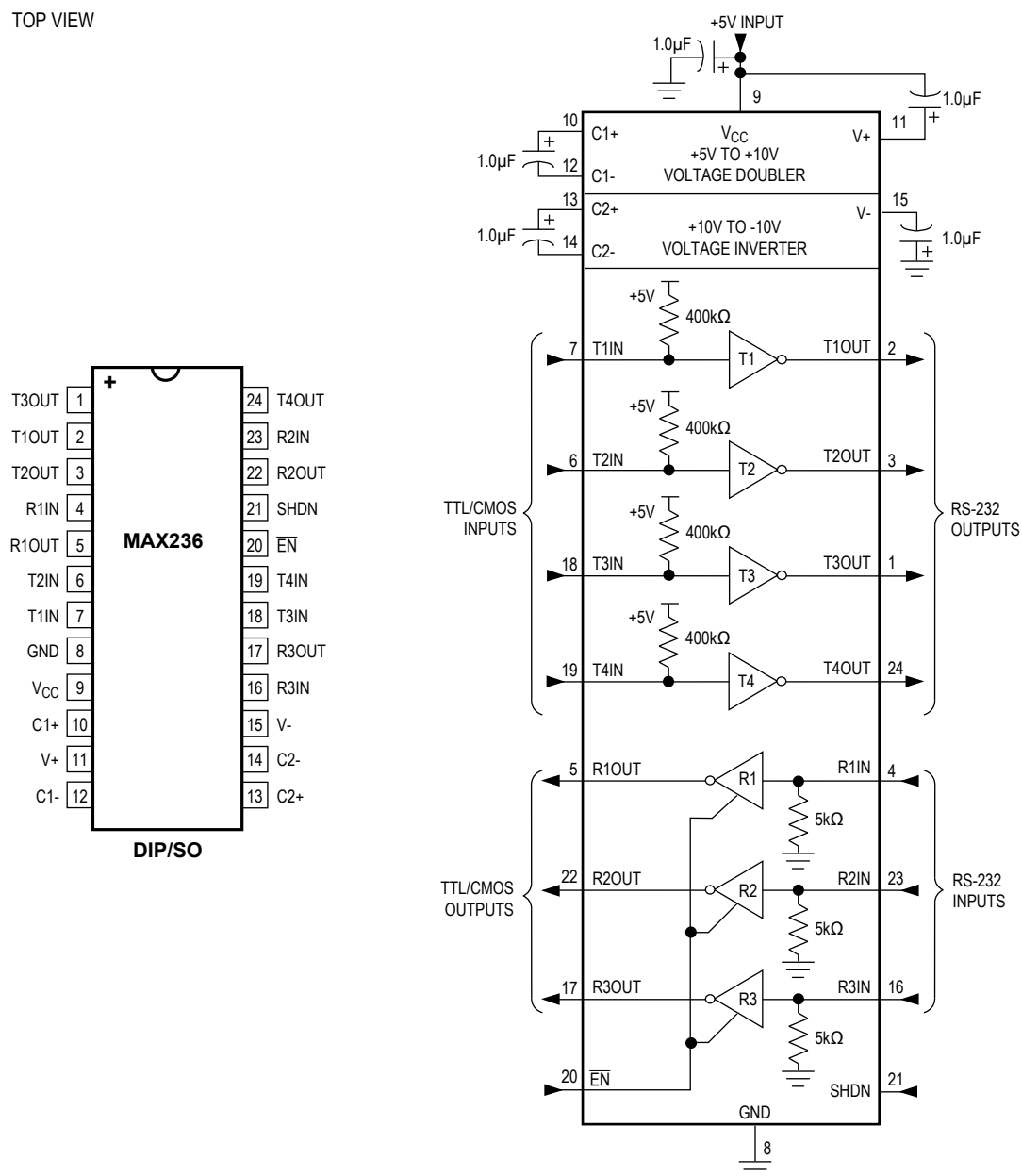
Figure 14. MAX246 Pin Configuration and Typical Operating Circuit
