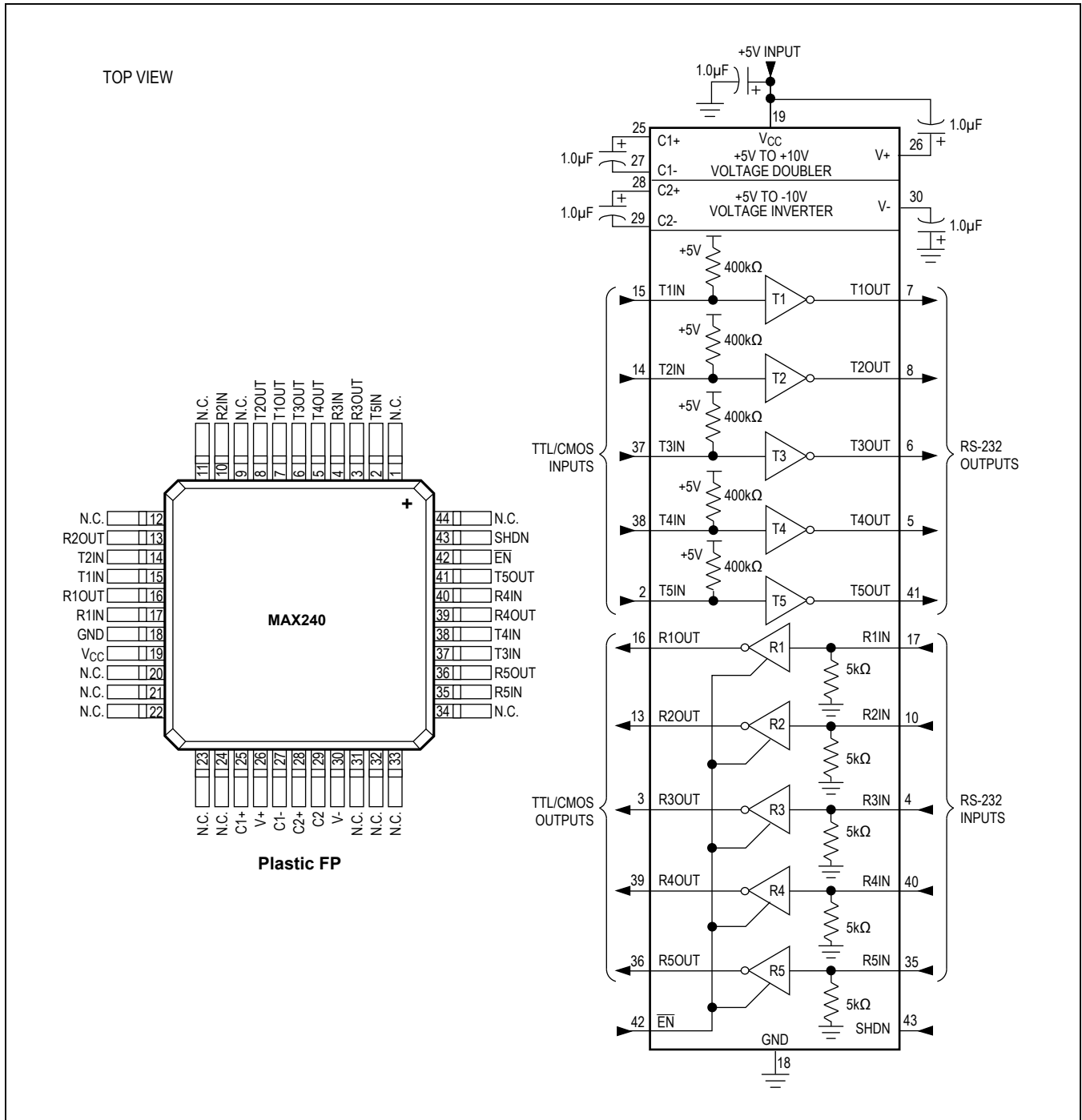
Figure 18. MAX244 Pin Configuration and Typical Operating Circuit
