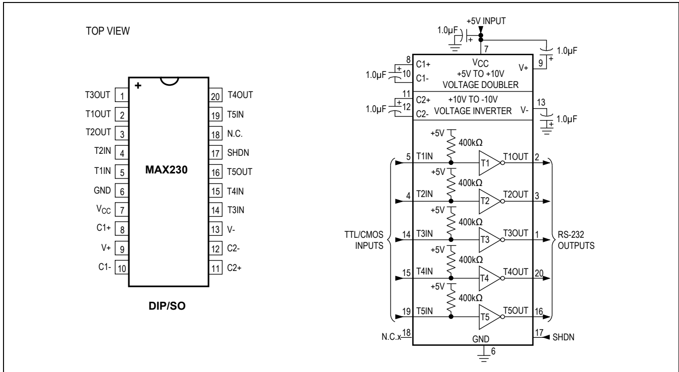
Figure 9. MAX238 Pin Configuration and Typical Operating Circuit
