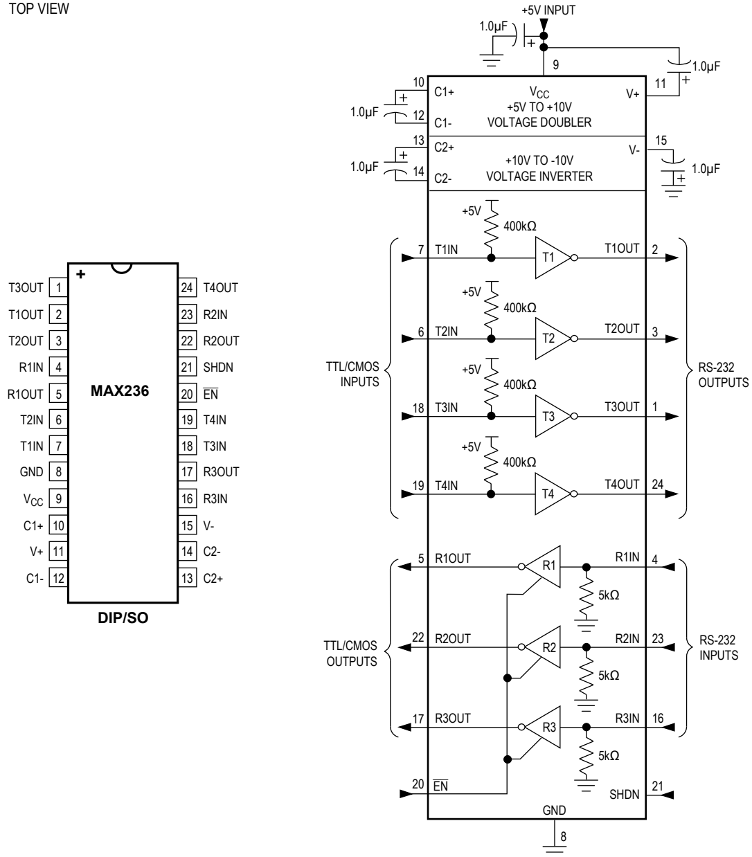
TOP VIEW
