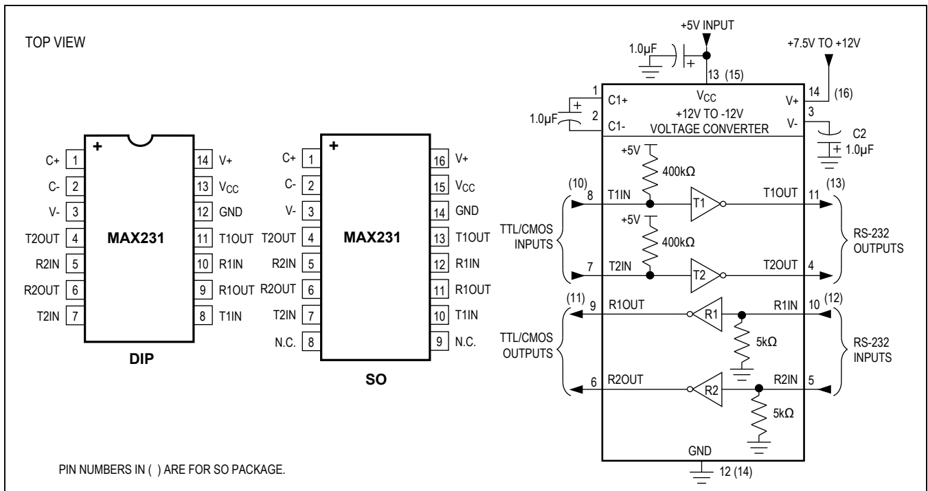
Figure 10. MAX2331 Pin Configurations and Typical Operating Circuit
