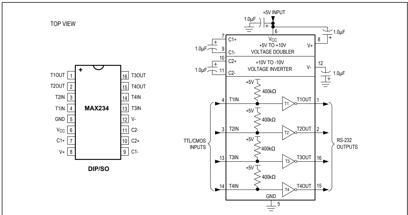
Figure 12. MAX2334 Pin Configuration and Typical Operating Circuit
