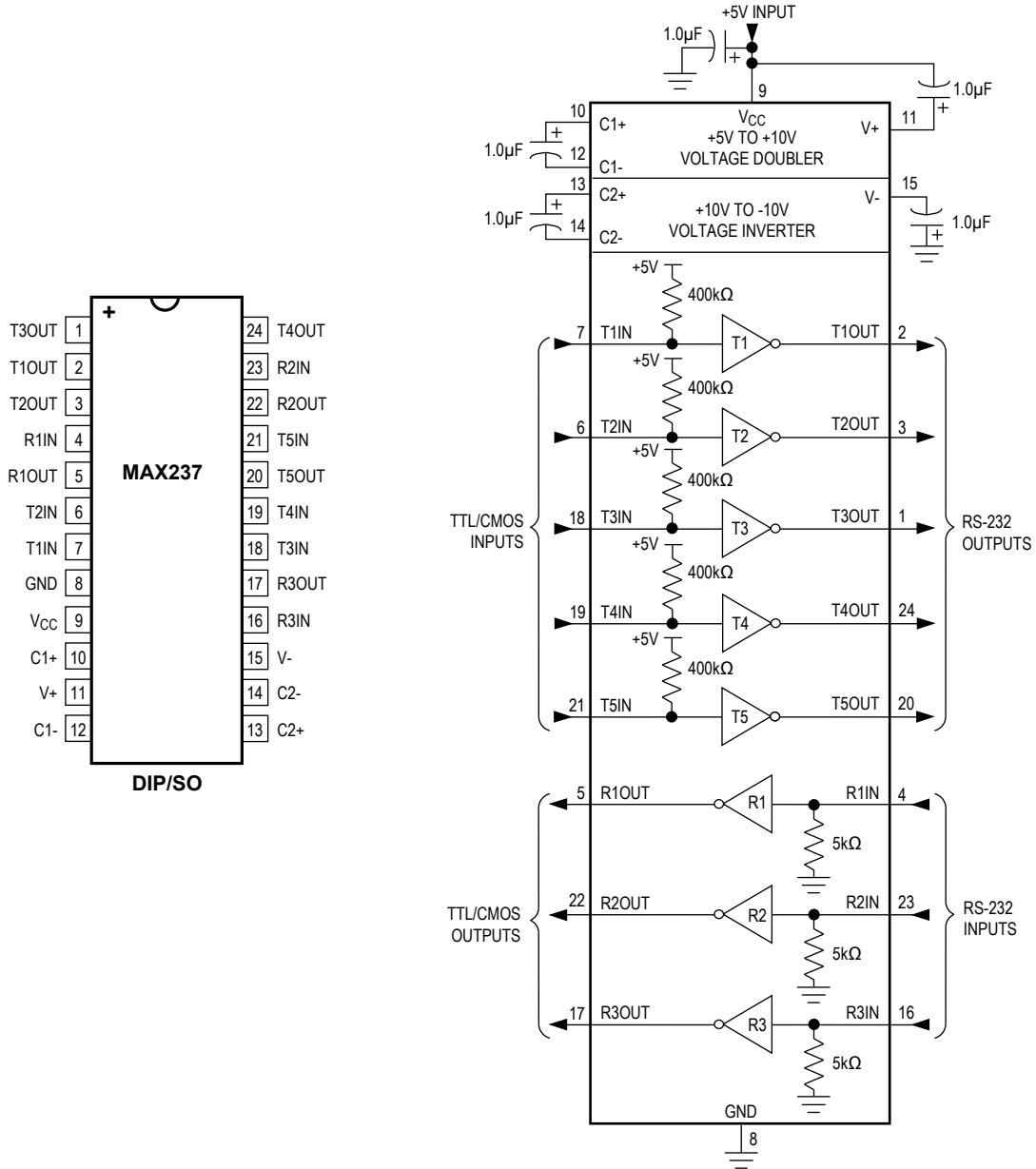
Figure 15. MAX233 Pin Configuration and Typical Operating Circuit
