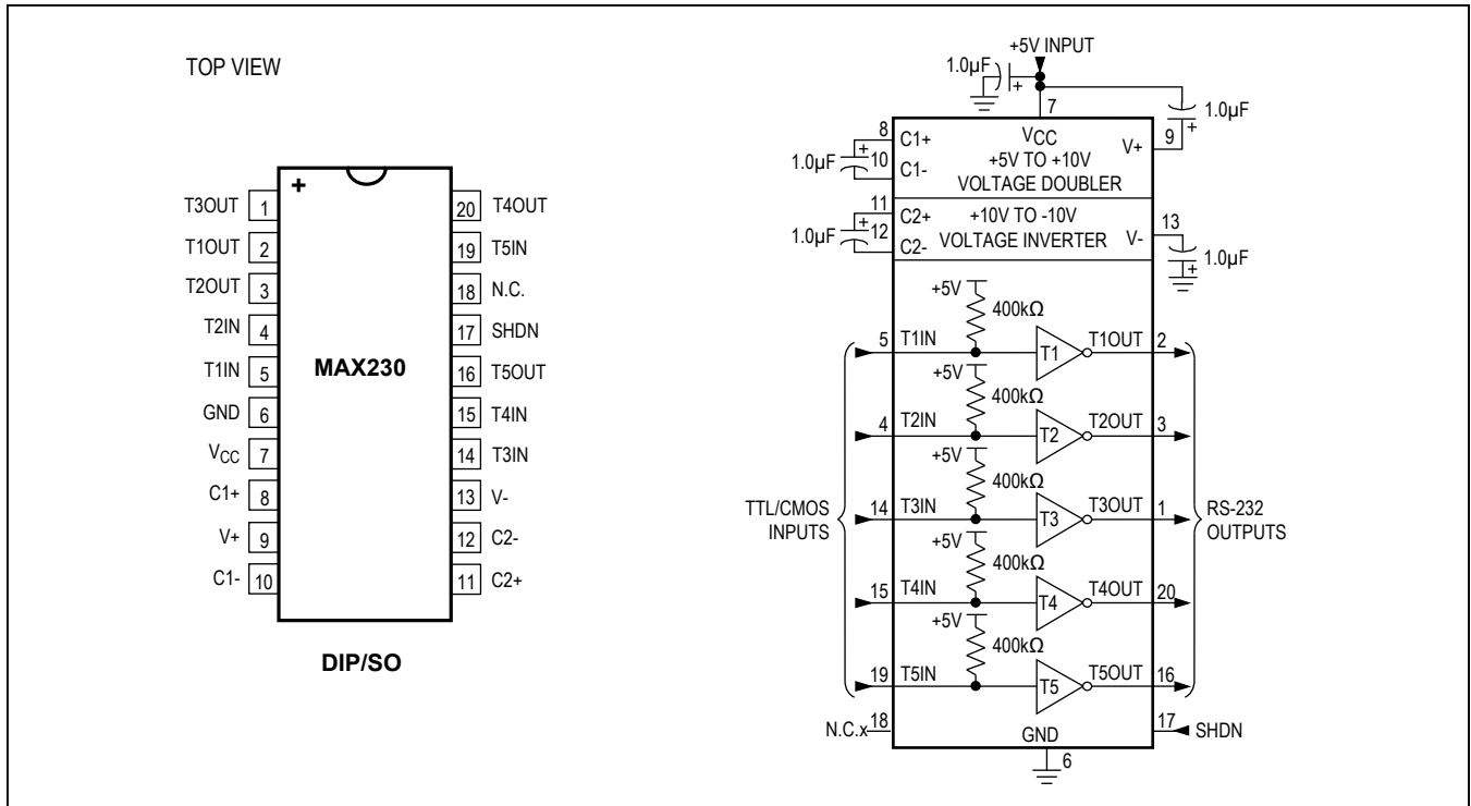
Figure 9. MAX233A Pin Configuration and Typical Operating Circuit
