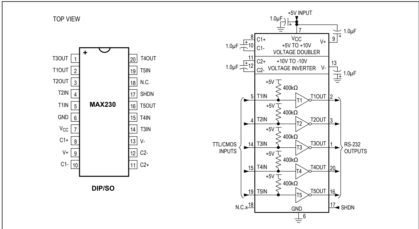
Figure 9. MAX233 Pin Configuration and Typical Operating Circuit
