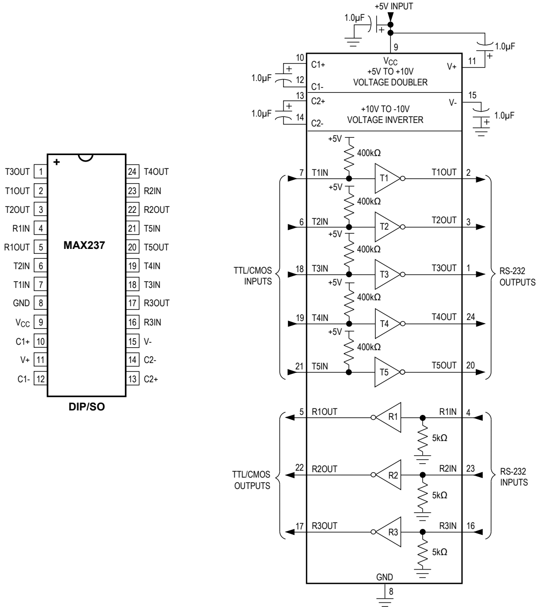
Figure 15. MAX232A Pin Configuration and Typical Operating Circuit
