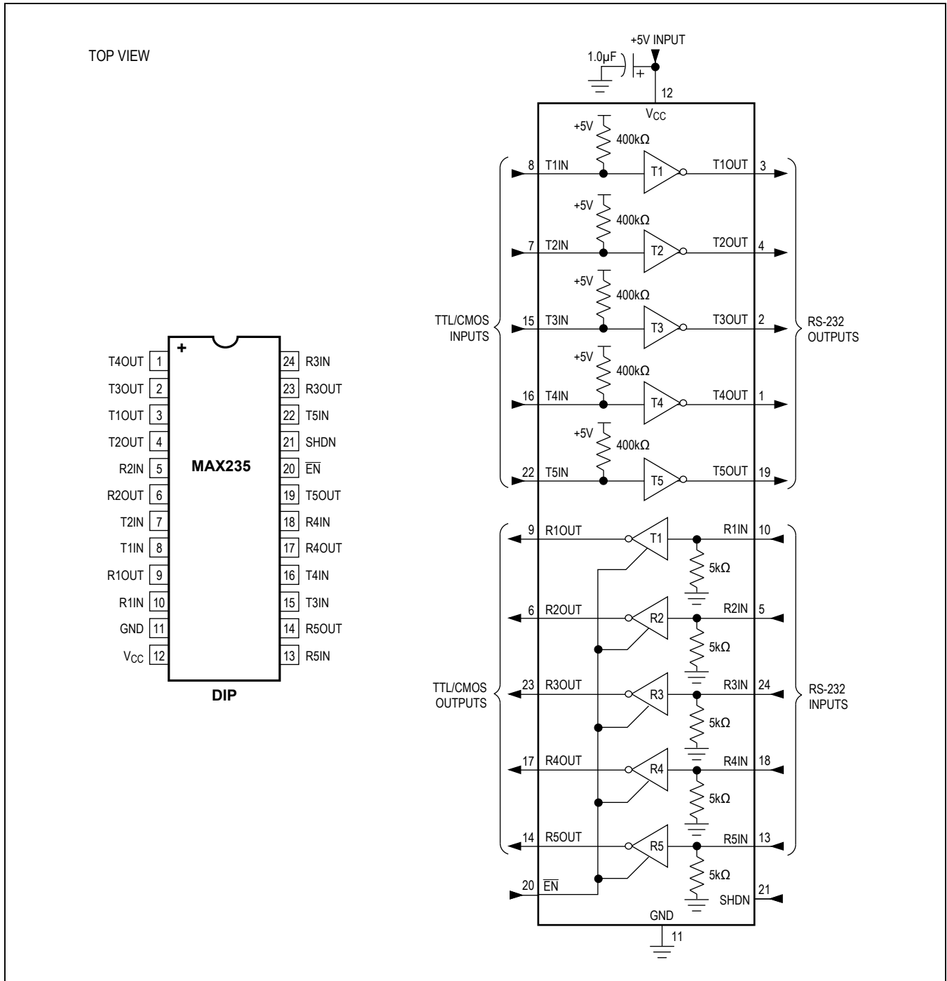
Figure 13. MAX232A Pin Configuration and Typical Operating Circuit
