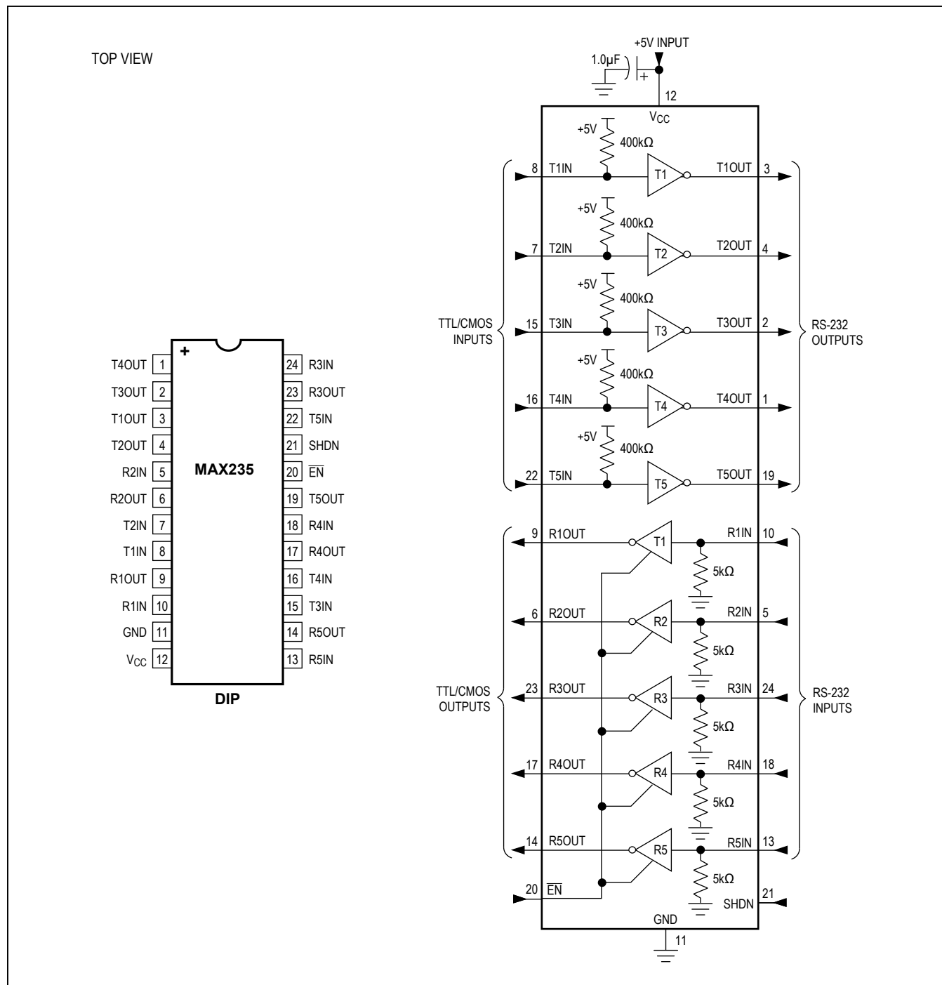
Figure 13. MAX231 Pin Configuration and Typical Operating Circuit
