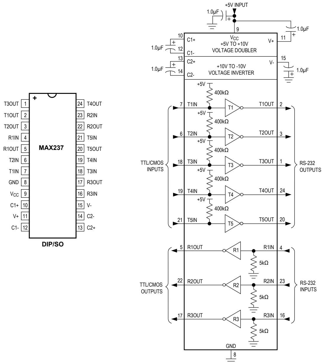
Figure 15. MAX230 Pin Configuration and Typical Operating Circuit
