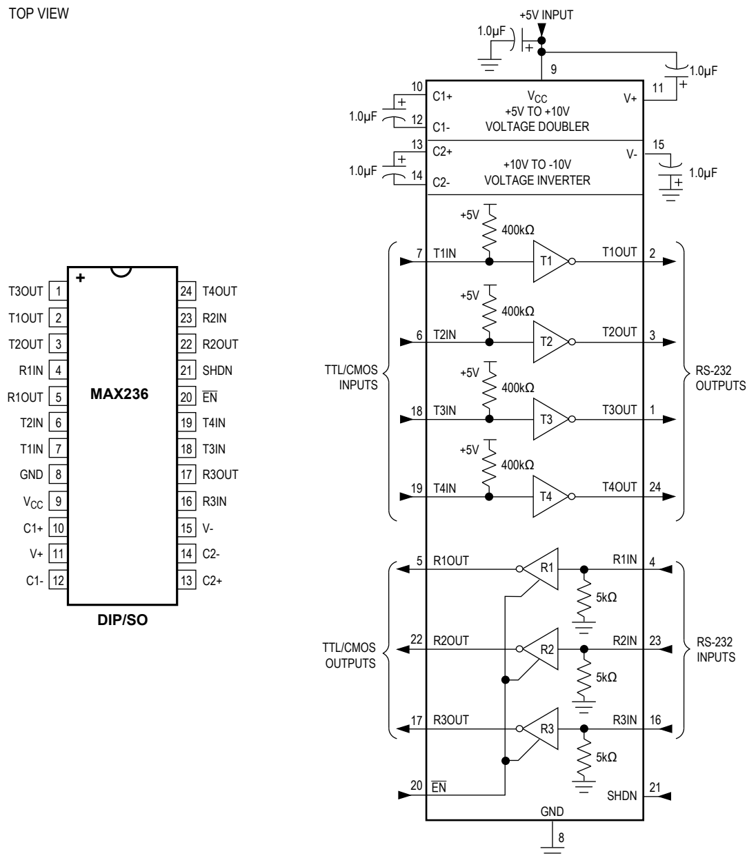
Figure 14. MAX236 Pin Configuration and Typical Operating Circuit
