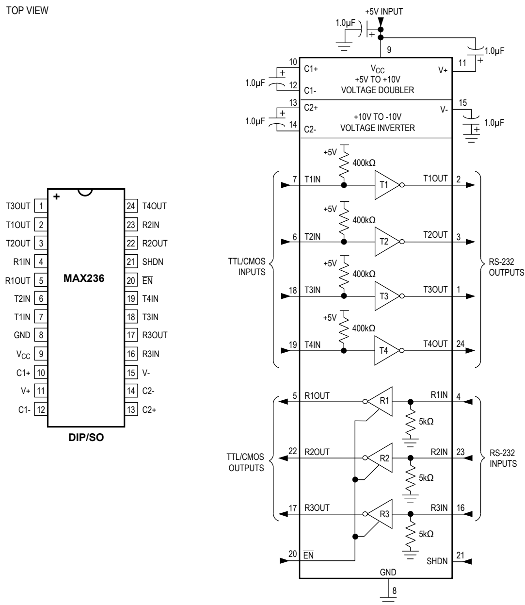
Figure 14. MAX220 Pin Configuration and Typical Operating Circuit
