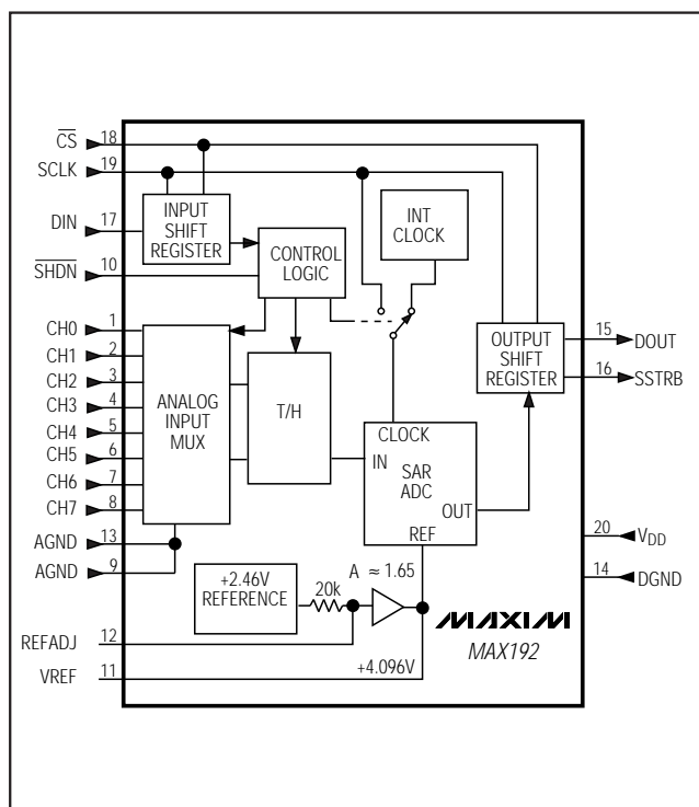
Figure 3. Block Diagram
