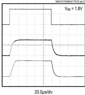
DYNAMIC OUTPUT-VOLTAGE TRANSIENT
