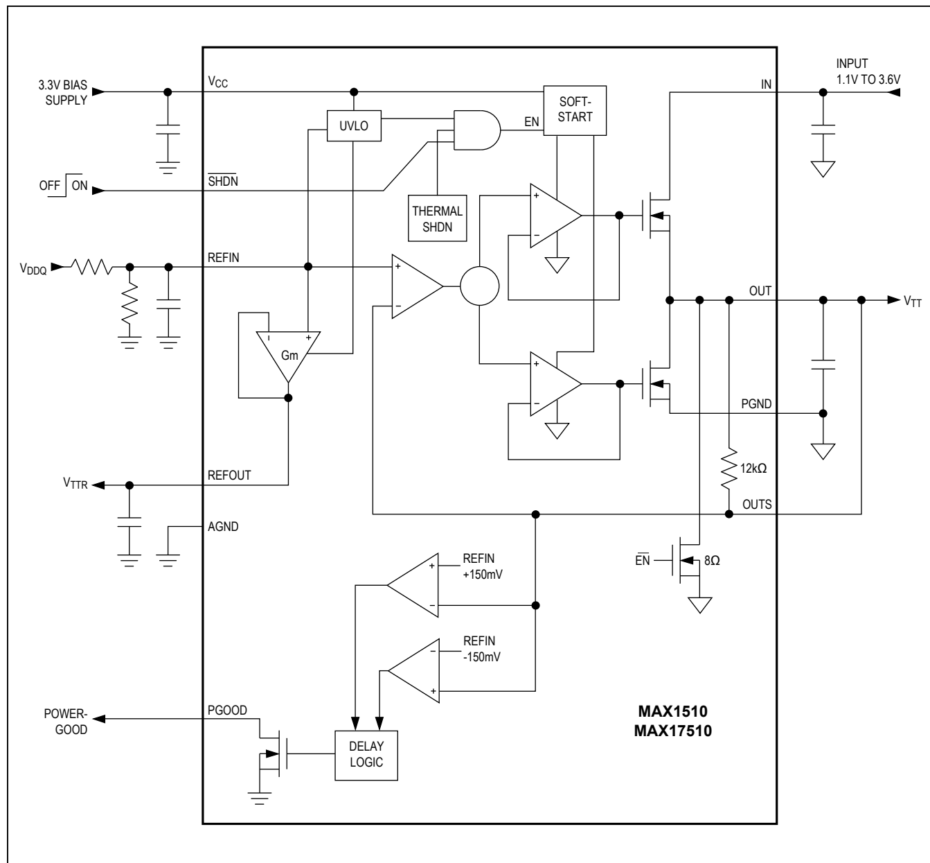
Figure 2. Functional Diagram
