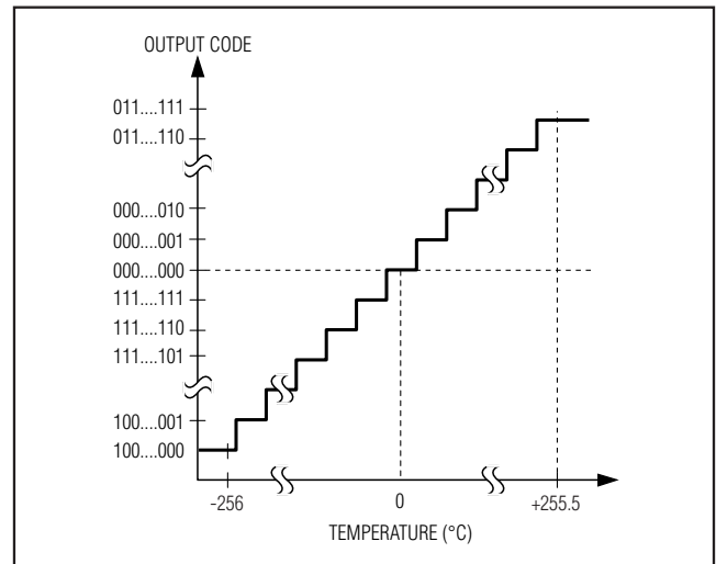
Figure 5. Temperature Transfer Function
