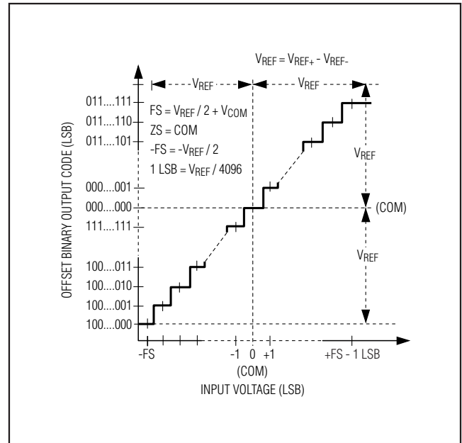
Figure 4. Bipolar Transfer Function—Full Scale ( \pm\text{FS} ) = \pm V_{\text{REF}} / 2
