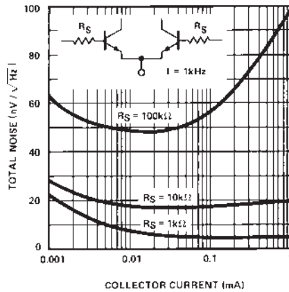
TPC 11. Total Noise vs. Collector Current
