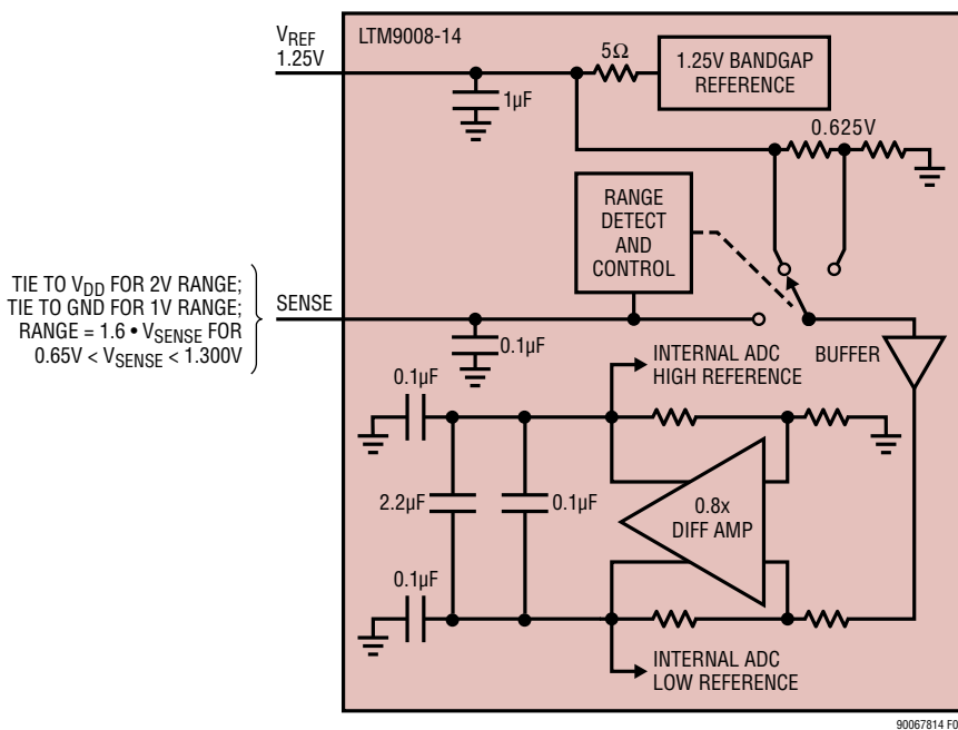
Figure 8. Reference Circuit
