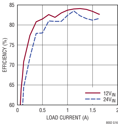
Efficiency, V_{OUT} = -12\text{V} , BIAS Tied to LTM8002 GND
