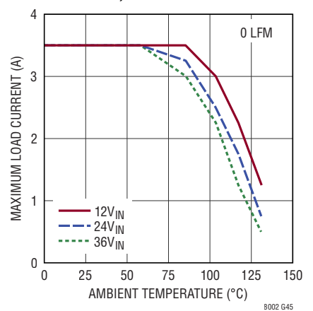
Derating, H-Grade, V_{\text{OUT}} = 2.5\text{V} , BIAS = 5V, DC2501A Demo Board
