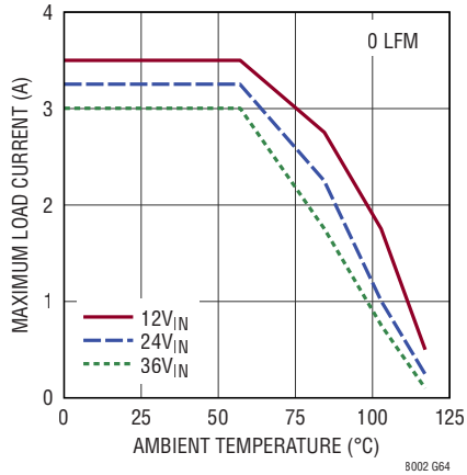
Derating, I-Grade, V_{OUT} = 2.5\text{V} , BIAS = 5V, DC2501A Demo Board
