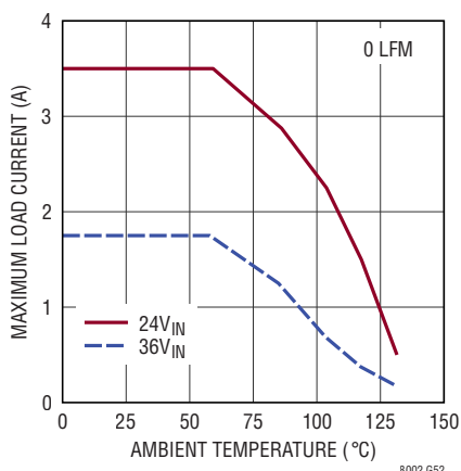
Derating, H-Grade, V_{OUT} = 18\text{V} , BIAS = 5V, DC2501A Demo Board
