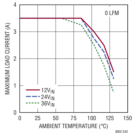
Derating, H-Grade, V_{\text{OUT}} = 1.5\text{V} , BIAS = 5V, DC2501A Demo Board
