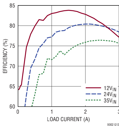
Efficiency, V_{OUT} = -3.3\text{V} , BIAS Tied to LTM8002 GND
