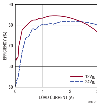
Efficiency, V_{OUT} = -5\text{V} , BIAS Tied to LTM8002 GND
