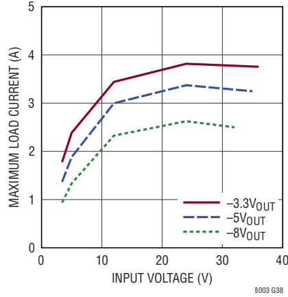
Maximum Load Current vs V_{\text{IN}} , BIAS Tied to LTM8002 GND
