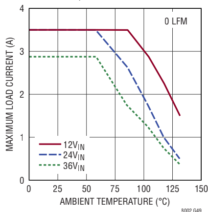
Derating, H-Grade, V_{OUT} = 8\text{V} , BIAS = 5V, DC2501A Demo Board
