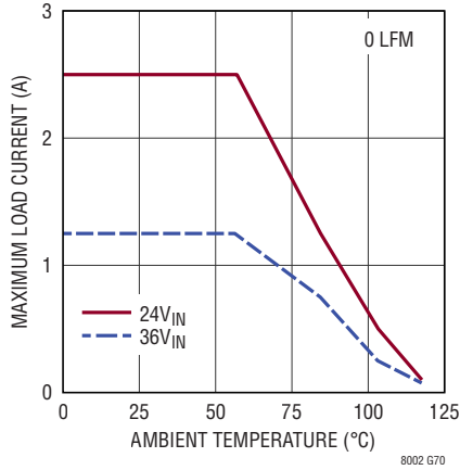
Derating, I-Grade, V_{OUT} = 12\text{V} , BIAS = 5V, DC2501A Demo Board
