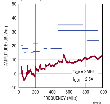
CISPR25 Class 5 Average Radiated DC2501A Demo Board, V_{OUT} = 5\text{V} Spread Spectrum Enabled
