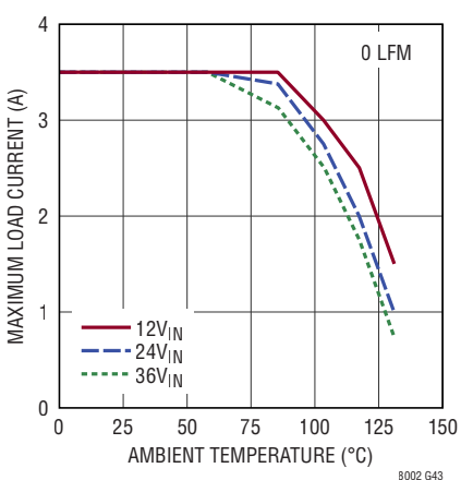
Derating, H-Grade, V_{\text{OUT}} = 1.8\text{V} , BIAS = 5V, DC2501A Demo Board
