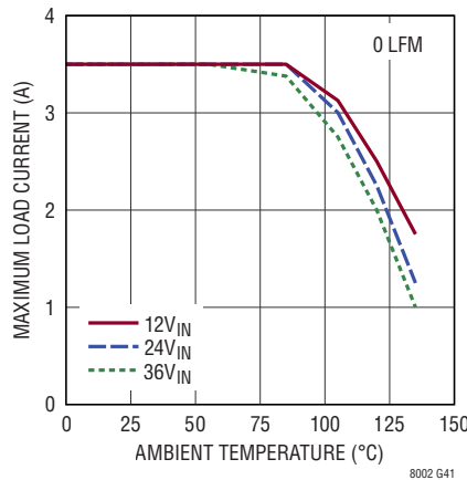
Derating, H-Grade, V_{\text{OUT}} = 1.2\text{V} , BIAS = 5V, DC2501A Demo Board
