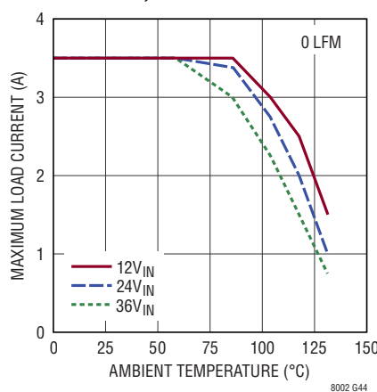
Derating, H-Grade, V_{\text{OUT}} = 2\text{V} , BIAS = 5V, DC2501A Demo Board
