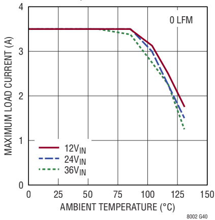
Derating, H-Grade, V_{\text{OUT}} = 0.97\text{V} , BIAS = 5V, DC2501A Demo Board
