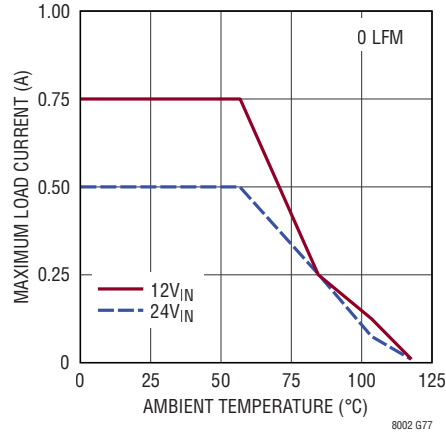
Derating, I-Grade, V_{OUT} = -15\text{V} , BIAS Tied to LTM8002 GND, DC2501A Demo Board
