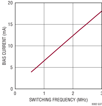
BIAS Current vs Frequency, 12\text{V}_{\text{IN}} , 5\text{V}_{\text{OUT}} , 2.5A Load SYNC Floating
