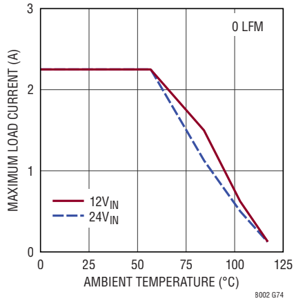
Derating, I-Grade, V_{OUT} = -5\text{V} , BIAS Tied to LTM8002 GND, DC2501A Demo Board
