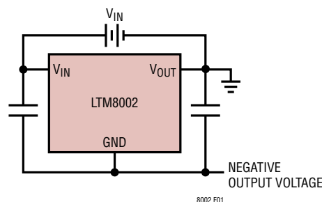
Figure 1. The LTM8002 Can Be Used to Generate a Negative Voltage
