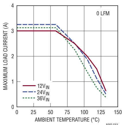
Derating, H-Grade, V_{OUT} = -3.3\text{V} , BIAS Tied to LTM8002 GND, DC2501A Demo Board
