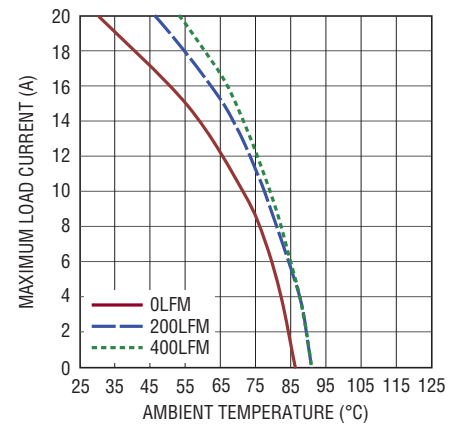
Figure 19. 12V to 1.8V Derating Curve, No Heat Sink
