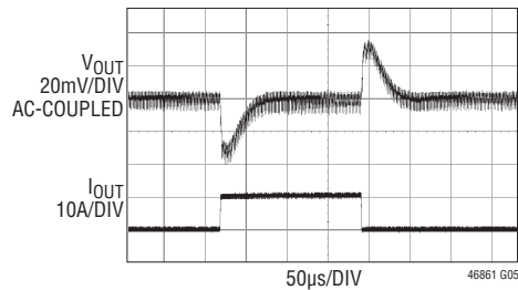
FIGURE 27 CIRCUIT AT 12\text{V}_{\text{IN}} . \text{INTV}_{\text{CC}} PIN OPEN CIRCUIT AND \text{VOUT\_COMMANDn} SET TO 1.000\text{V} . 10\text{A} TO 20\text{A} LOAD STEP AT 10\text{A}/\mu\text{s}
