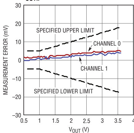
READ_VOUT _n (Output Voltage Readback) Error vs V_{\text{OUT}n} I_{\text{OUT}n} = No Load, \text{RUN}1-n = 0\text{V}
