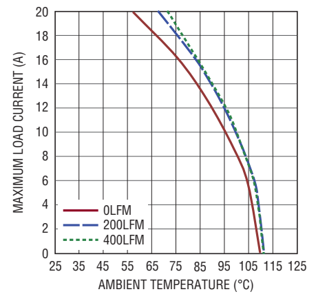
Figure 16. 5V to 1V Derating Curve, with Heat Sink
