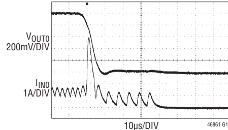
FIGURE 61 CIRCUIT AT 12\text{V}_{\text{IN}} . 100m \Omega LOAD ON V_{\text{OUT}0} PRIOR TO APPLICATION OF SHORT CIRCUIT
