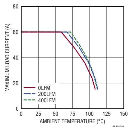
Figure 40. 12V to 0.9V Derating Curve, No Heat Sink
