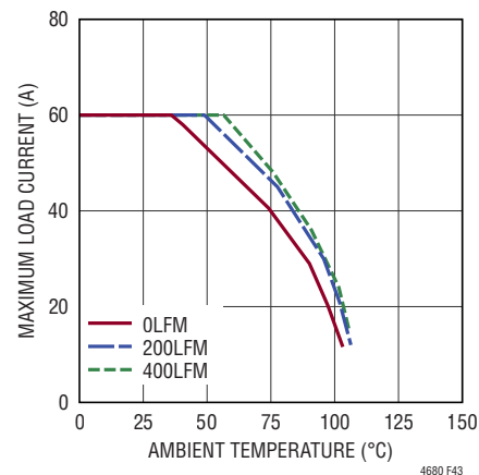
Figure 43. 12V to 1.8V Derating Curve, No Heat Sink
