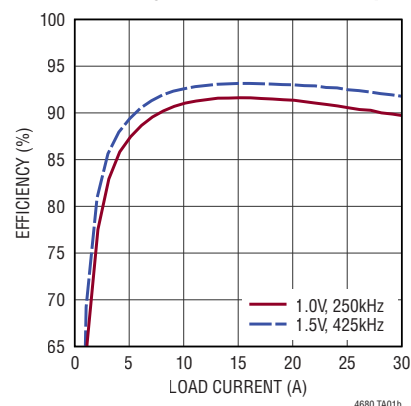
Efficiency vs Current at 12V Input
