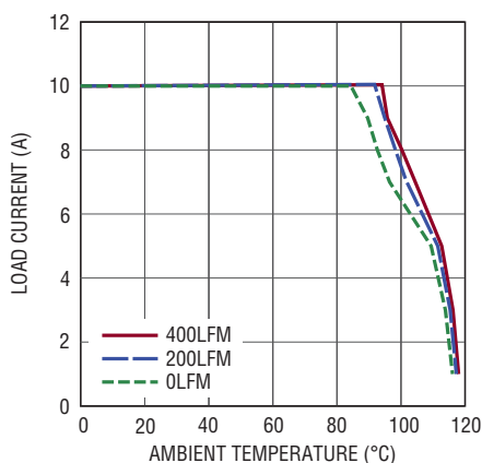
Figure 14. No Heat Sink with 5V_{IN} to 2.5V_{OUT}
