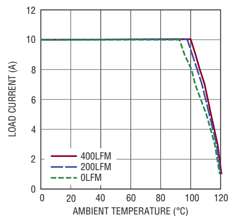
Figure 13. No Heat Sink with 3.3V_{IN} to 2.5V_{OUT}
