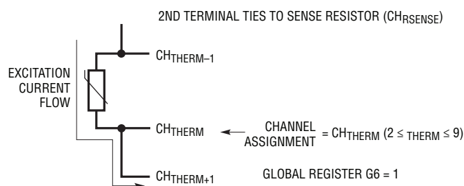
Figure 45. Thermistor Kelvin Current Source Mode (G6 = 1)
