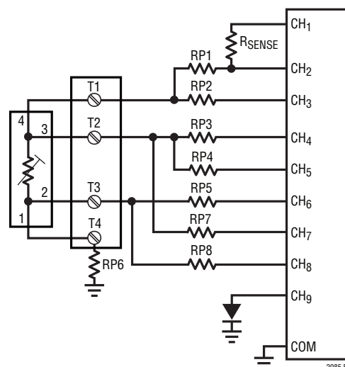
Figure 48. Protected Multi-Sensor 4-Wire RTD Connection
