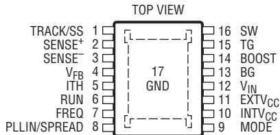
MSE PACKAGE 16-LEAD PLASTIC MSOP
