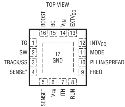
UD PACKAGE 16-LEAD (3mm × 3mm) PLASTIC QFN
