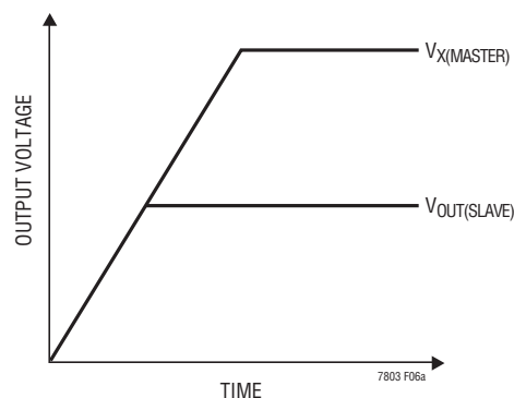
(6a) Coincident Tracking
