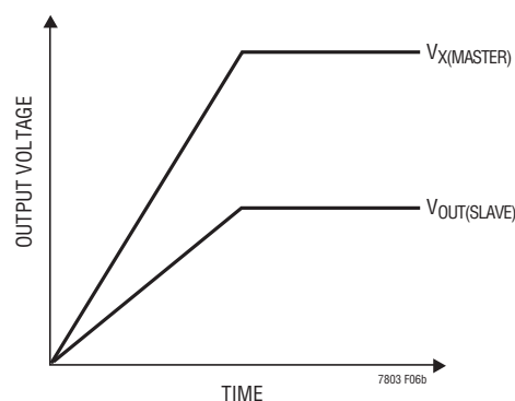
(6b) Ratiometric Tracking
