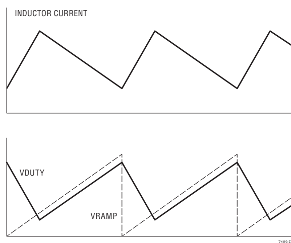
Figure 1. Typical Current Loop Operating Waveforms
