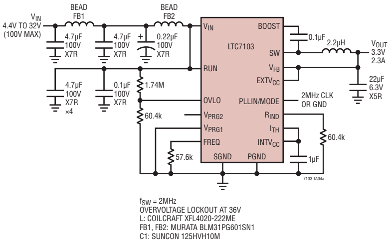
4.4V to 32V Input to 3.3V/2.3A Output, 2MHz Automotive Supply with Overvoltage Lockout and 100V Input Tolerance
