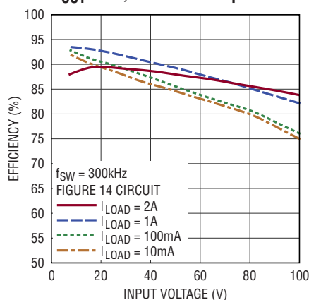
Efficiency vs Input Voltage V_{OUT} = 5\text{V} , Burst Mode Operation
