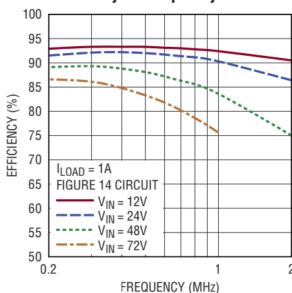
Efficiency vs Frequency at 1\text{A}
