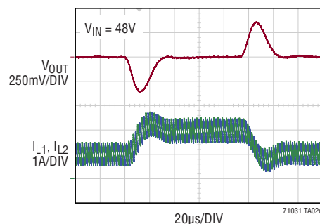
Load Transient
