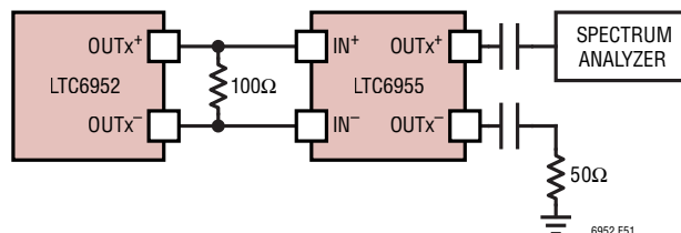
Figure 51. Example of Spurious Measurement Technique
