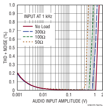
LTC6262 Bridge Driver THD and Noise with Different Loads vs Amplitude at 1kHz
