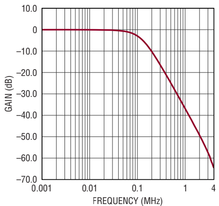
LTC6261 Second Order Butterworth Frequency Response
