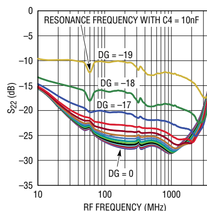
RF Return Loss
