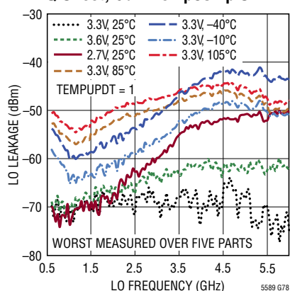
LO Leakage vs LO Frequency After 25°C, 3.3V Calibration Using I and Q Offset, Gain TempComp Off
