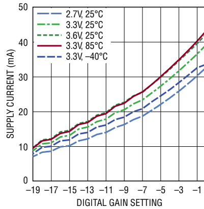
Supply Current vs Digital Gain Setting
