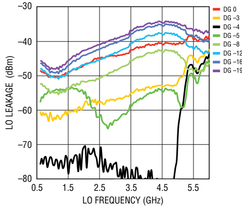
LO Leakage vs LO Frequency and Digital Gain Setting After Calibration Using Reg. 0x02 and 0x03 at Digital Gain = -4
