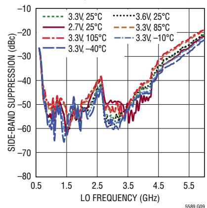
Side-Band Suppression vs LO Frequency for Gain TempComp On
