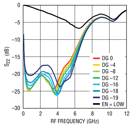
RF Return Loss
