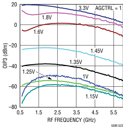
Output IP3 vs RF Frequency and V_{CTRL}
