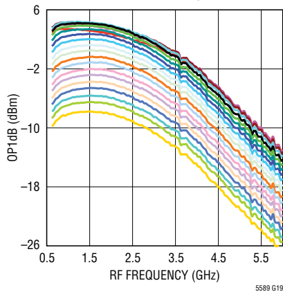
Output 1dB Compression Point vs RF Frequency and Digital Gain Setting at 3.3V Supply, 85°C
