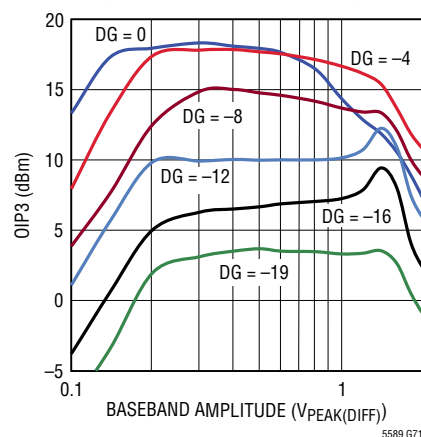
Output IP3 vs Baseband Amplitude
