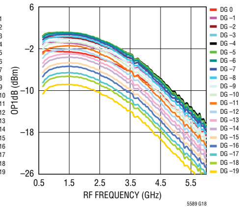
Output 1dB Compression Point vs RF Frequency and Digital Gain Setting at 2.7V Supply, 85^\circ C
