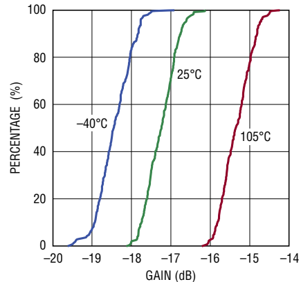
Gain Cumulative Distribution for V_{CTRL} = 1.75V
