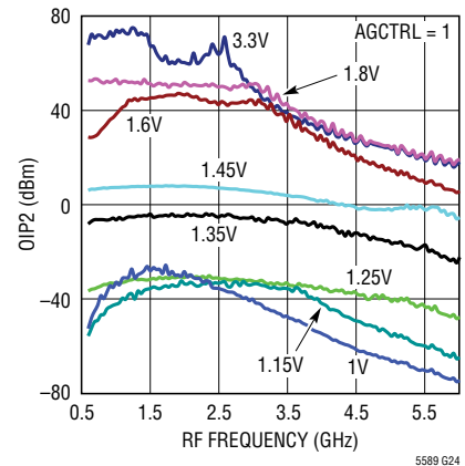
Output IP2 vs RF Frequency and V_{CTRL}
