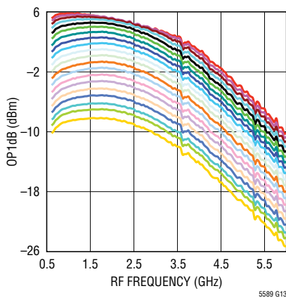
Output 1dB Compression Point vs RF Frequency and Digital Gain Setting at 2.7V Supply, -10^\circ C
