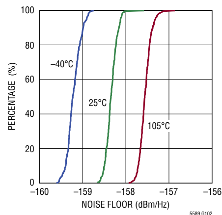
Output Noise Floor Cumulative Distribution
