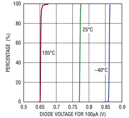
Temperature Sensing Diode Voltage Cumulative Distribution
