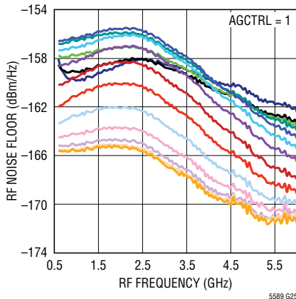
Noise Floor vs RF Frequency and V_{CTRL}
