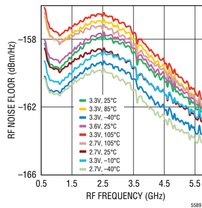
Noise Floor vs RF Frequency
