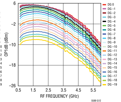
Output 1dB Compression Point vs RF Frequency and Digital Gain Setting at 3.3V Supply, -40^\circ C
