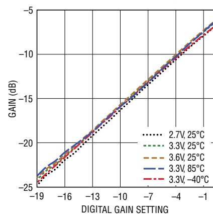
Gain vs Digital Gain Setting
