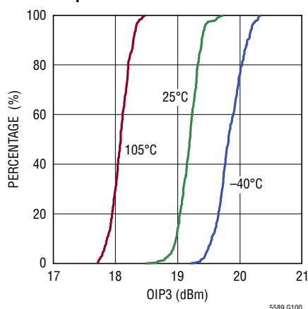
Output IP3 Cumulative Distribution
