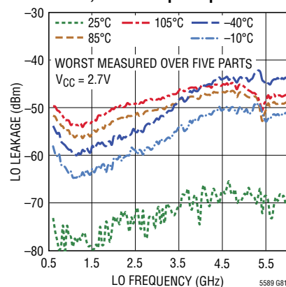
LO Leakage vs LO Frequency After 25°C, 2.7V Calibration Using I and Q Offset, Gain TempComp On
