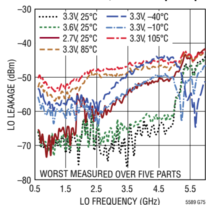
LO Leakage vs LO Frequency After 25°C, 3.3V Calibration Using Reg. 0x02 and 0x03, Gain TempComp On
