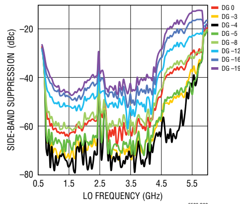
Side-Band Suppression vs LO Frequency and Digital Gain Setting After Calibration at Digital Gain = -4
