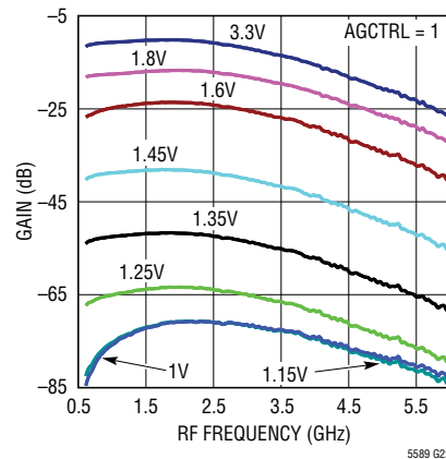
Gain vs RF Frequency and V_{CTRL}
