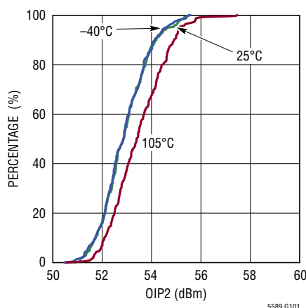
Output IP2 Cumulative Distribution
