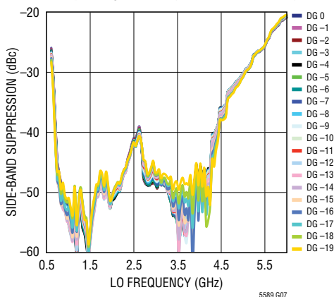
Side-Band Suppression vs LO Frequency and Digital Gain Setting
