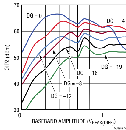
Output IP2 vs Baseband Amplitude
