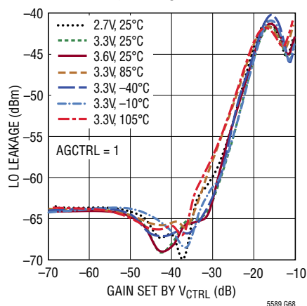
LO Leakage vs V_{CTRL} Gain
