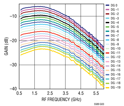
Gain vs RF Frequency and Digital Gain Setting
