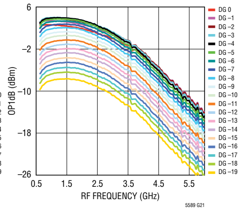
Output 1dB Compression Point vs RF Frequency and Digital Gain Setting at 3.3V Supply, 105°C
