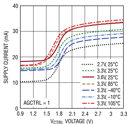
Supply Current vs V_{CTRL} Voltage
