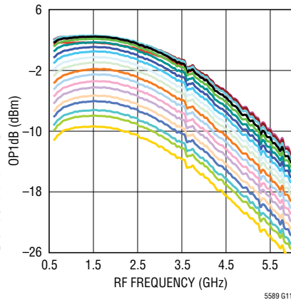
Output 1dB Compression Point vs RF Frequency and Digital Gain Setting at 2.7V Supply, -40^\circ C
