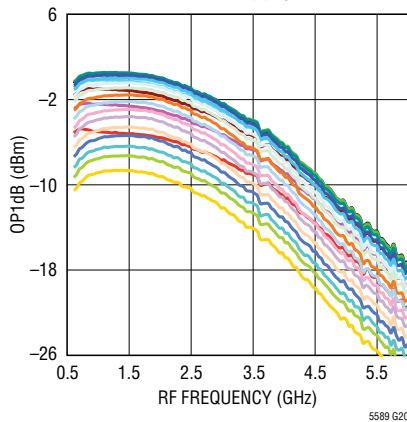
Output 1dB Compression Point vs RF Frequency and Digital Gain Setting at 2.7V Supply, 105°C
