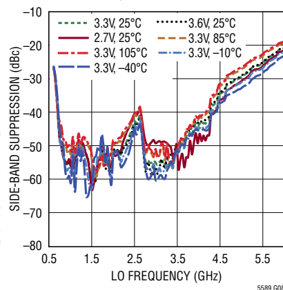
Side-Band Suppression vs LO Frequency for Gain TempComp Off
