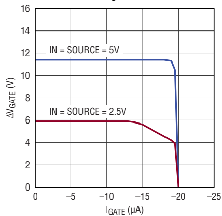
\Delta V_{\text{GATE}} (Average) vs GATE Leakage
