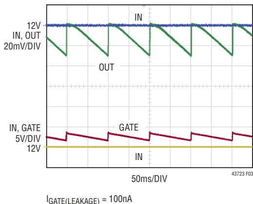
Figure 3. Regulating \Delta V_{SD} at Low I_{LOAD} = 1\mu\text{A}
