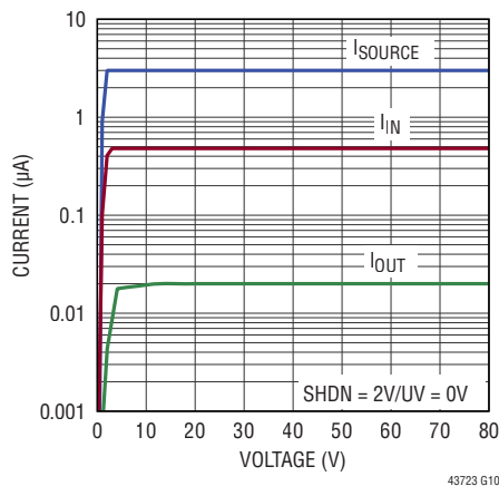
Pin Current at Shutdown
