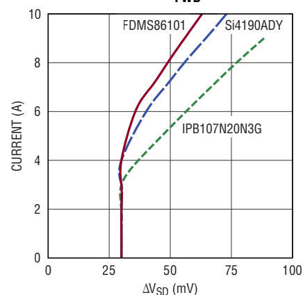
Load Current vs V_{\text{FWD}}
