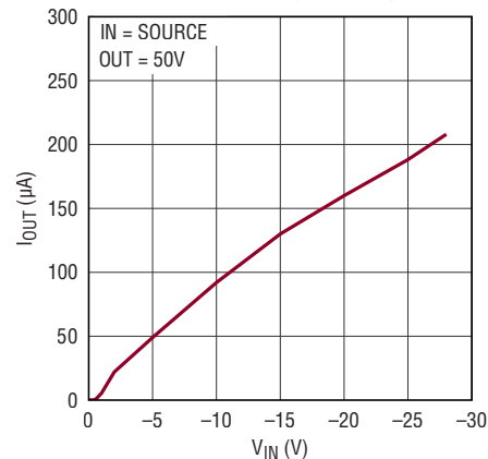
OUT Current at Negative Input
