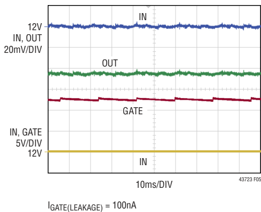
Figure 5. Regulating \Delta V_{GATE} at High I_{LOAD} = 16\text{A}
