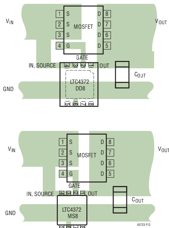
Figure 12. Layout, MS8 and DD8 Package
