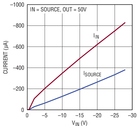
Pin Current at Negative Input
