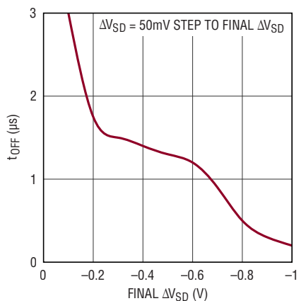
GATE Turn-Off Time vs Forward Overdrive
