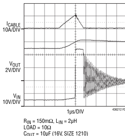
Figure 7. Overvoltage Protection Waveforms When 20V Plugged into 5V System
