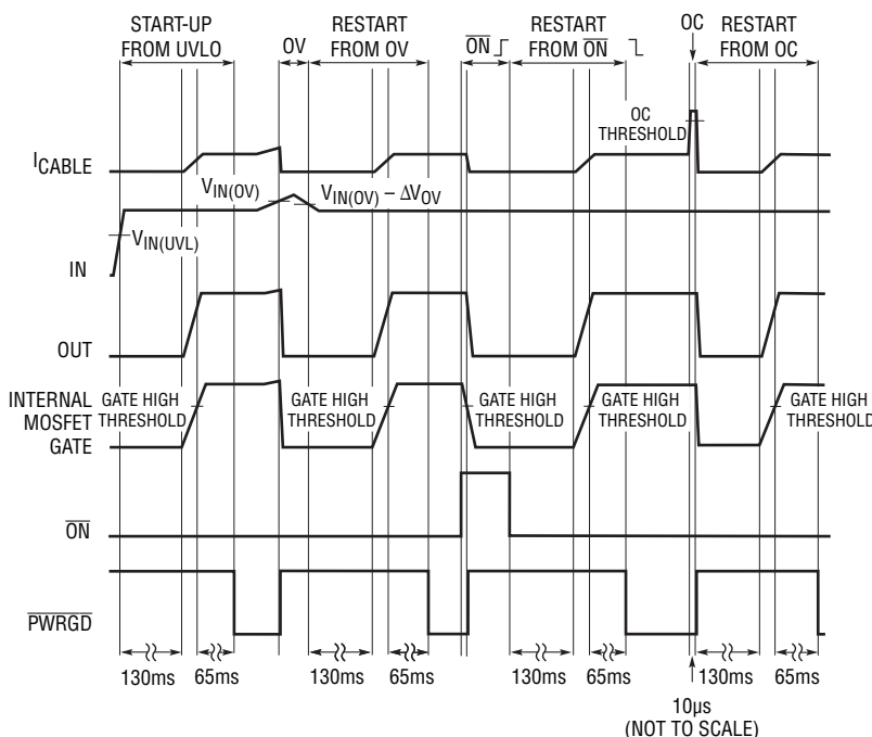
Figure 2. \overline{\text{PWRGD}} Behavior
