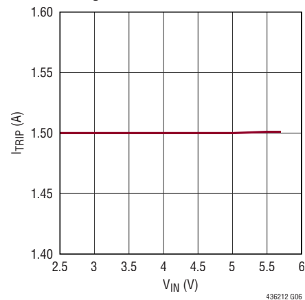
Overcurrent Threshold vs Input Voltage
