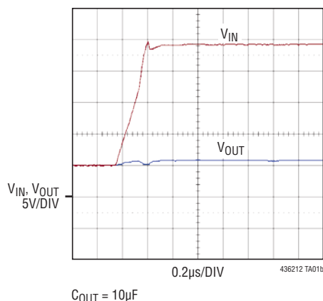
Output Protected from Overvoltage at Input
