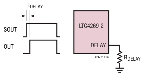
Figure 14. Programming SOUT and OUT Delay: t_{\text{DELAY}}
