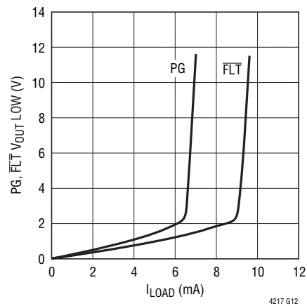
PG, \overline{\text{FLT}} V_{OUT} Low vs I_{LOAD}
