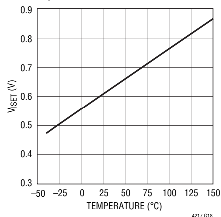
V_{\text{ISSET}} vs Temperature
