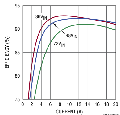
12V OUT , 240W Converter Efficiency
