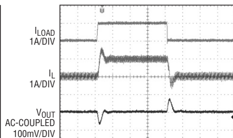
Load Step, Forced Continuous Operation
