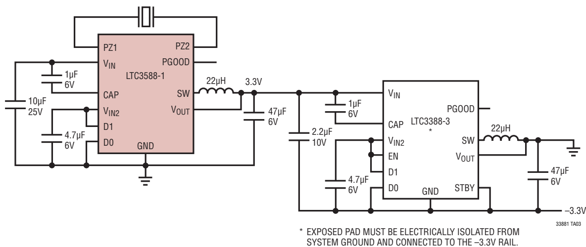
Figure 13. Piezoelectric Energy Harvester with \pm 3.3\text{V} Outputs
