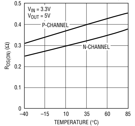
N-Channel and P-Channel R_{DS(ON)}
